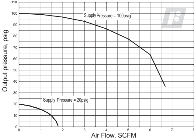
Flow Characteristics Fairchild Model 90052
